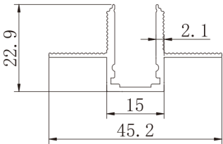
RECESSED MAGENTIC TRACK AX1020-N
